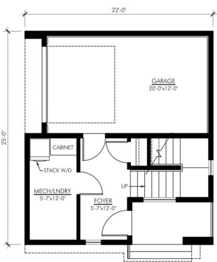
MAIN FLOOR PLAN - 239 SQ FT ASHLEY - 754
