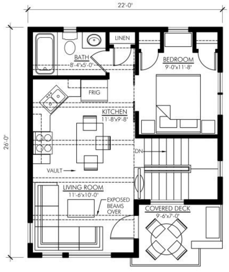
SECOND FLOOR PLAN - 515 SQ FT ASHLEY - 754
