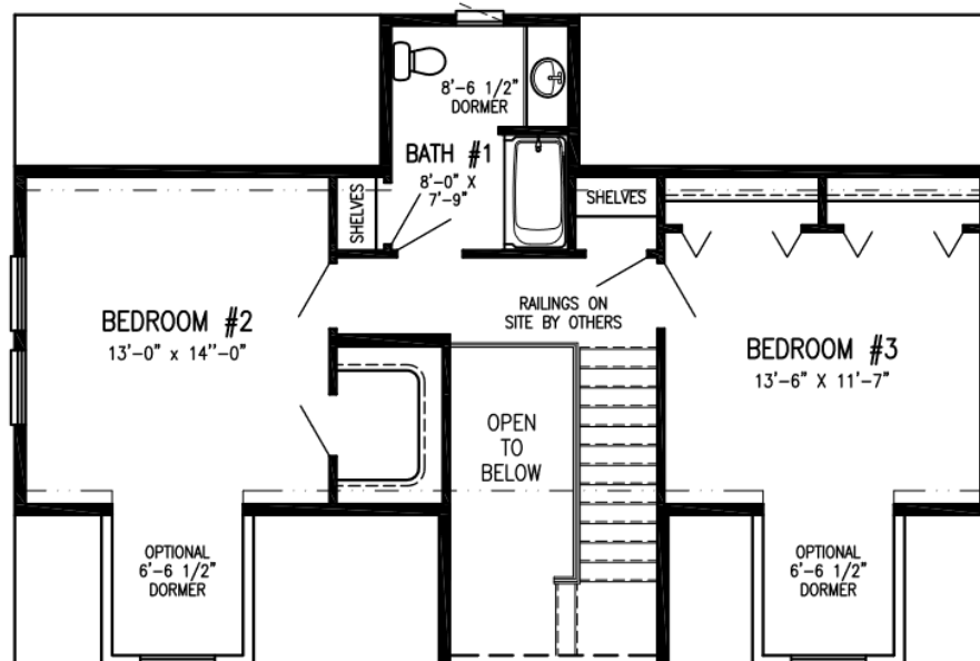
Second Floor
