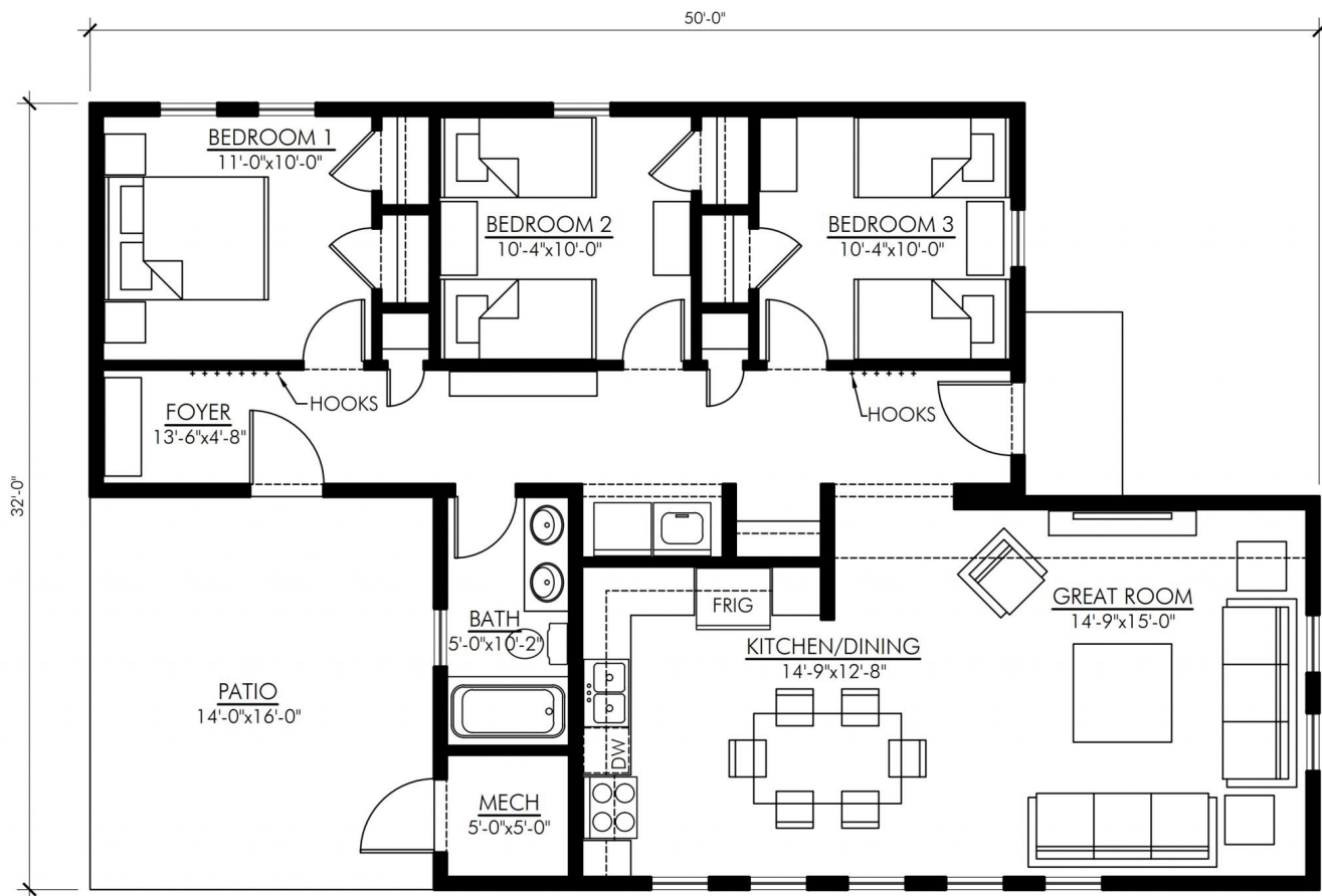
MAIN FLOOR PLAN CARIBOU-1184
