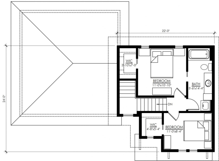
SECOND FLOOR PLAN - 473 SQ. FT. AUSTRING - 946G
