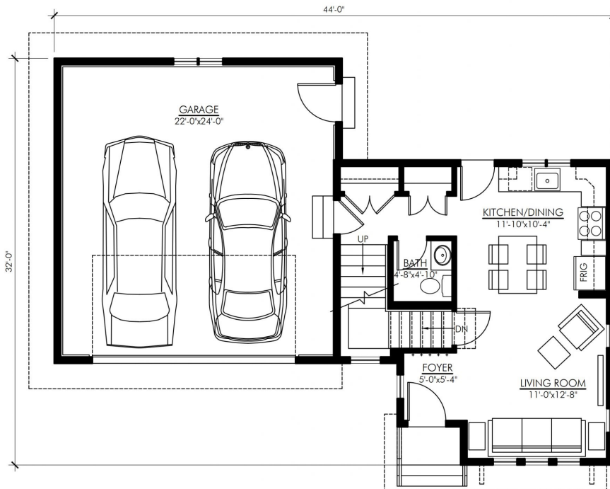
MAIN FLOOR PLAN - 473 SQ. FT. AUSTRING - 946G
