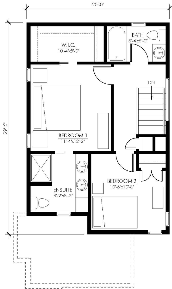
SECOND FLOOR PLAN - 569 SQ. FT. ASCEND - 1285
