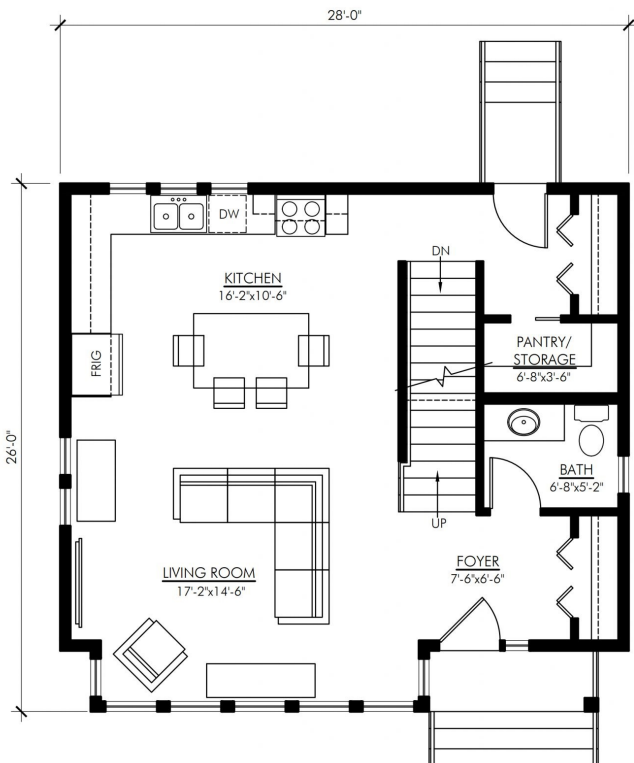
MAIN FLOOR PLAN - 694 SQ FT ALEXANDER - 1338
