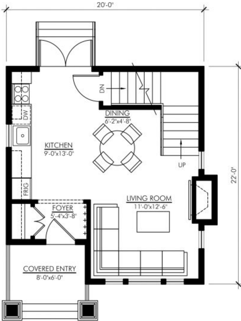
MAIN FLOOR PLAN - 415 SQ FT WINDSOR - 673
