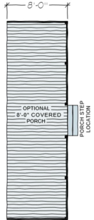
Porch Option
