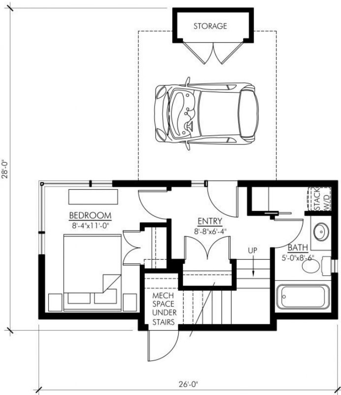
MAIN FLOOR PLAN - 324 SQ FT MANITOBA-636
