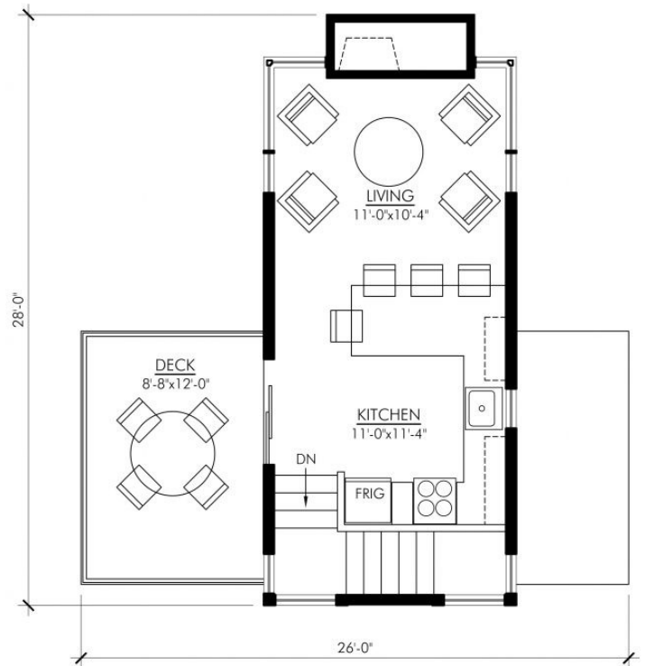
SECOND FLOOR PLAN - 312 SQ FT MANITOBA-636
