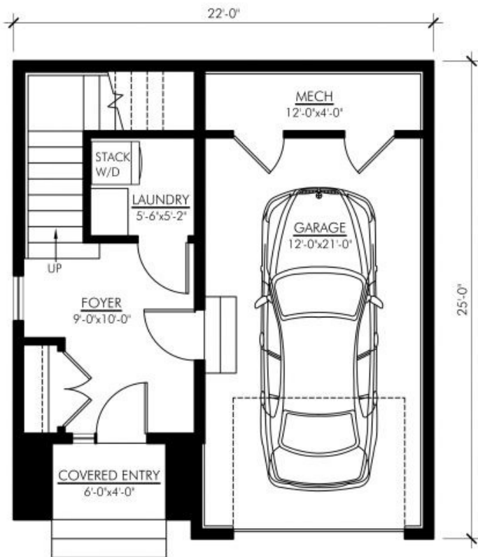
MAIN FLOOR PLAN - 200 SQ FT DURUM - 728
