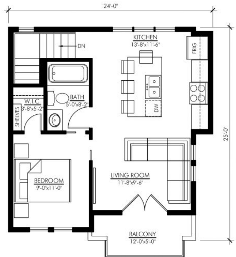
SECOND FLOOR PLAN - 528 SQ FT DURUM - 728
