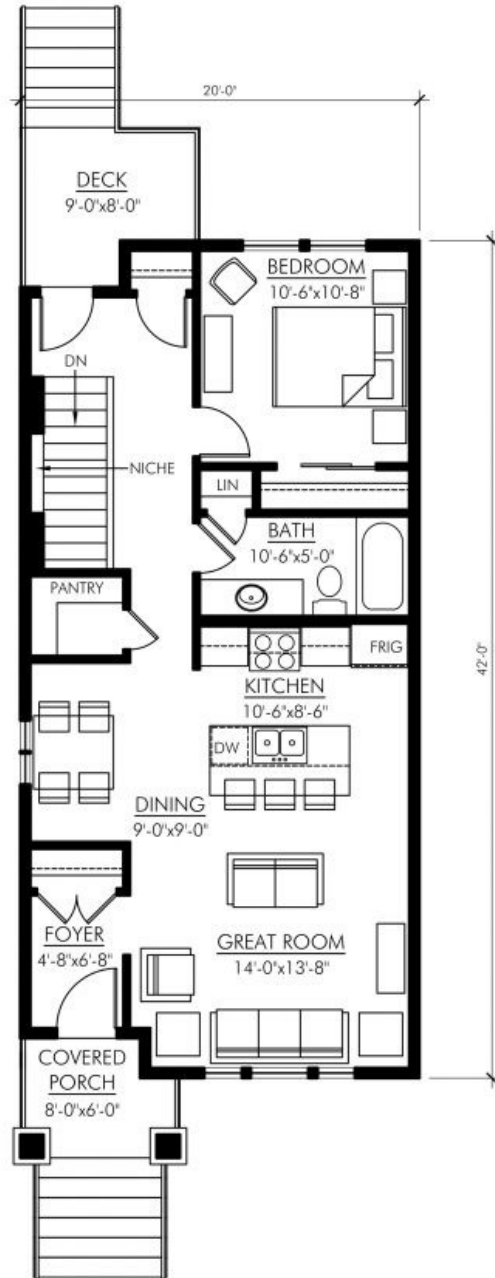
MAIN FLOOR PLAN - 816 SQ FT BRODER-816
