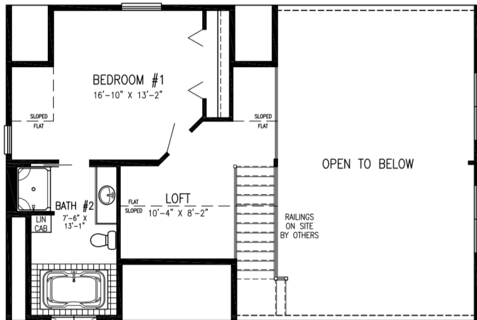
Second Floor (Bonus Room)
